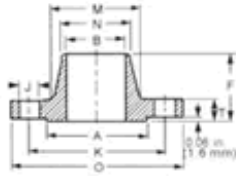
WELDING NECK
